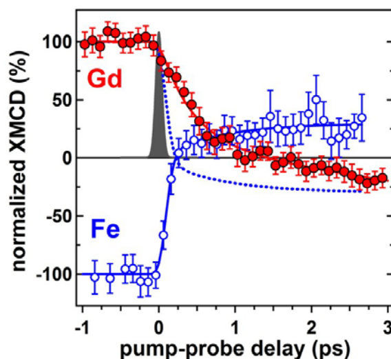
Fig. 2 (adapted from [9]) Divergent dynamics of the Fe and Gd magnetic moments measured by time-resolved XMCD with fs time-resolution within the first 3 ps. Experimental time resolution of 100 fs is depicted by the solid Gaussian profile. The solid and dashed lines are guides to the eye. The dashed line depicts the magnetization of Fe-sublattice taken with the opposite sign.
