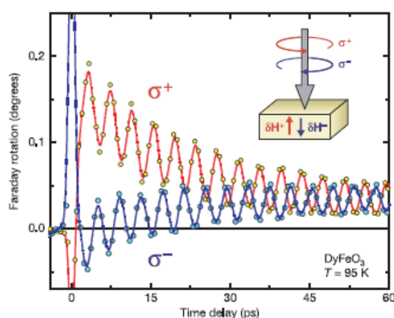
Fig. 1 Magnetic excitations in \text{DyFeO}_3 : the circularly polarized pumps of opposite helicities excite oscillations of opposite phase. Inset shows the geometry of the experiment. From reference [4]
