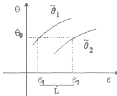
Fig. 5. Variation of free energy of the two phases.
