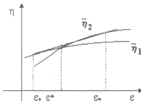
Fig. 4. Convexification of entropy.
